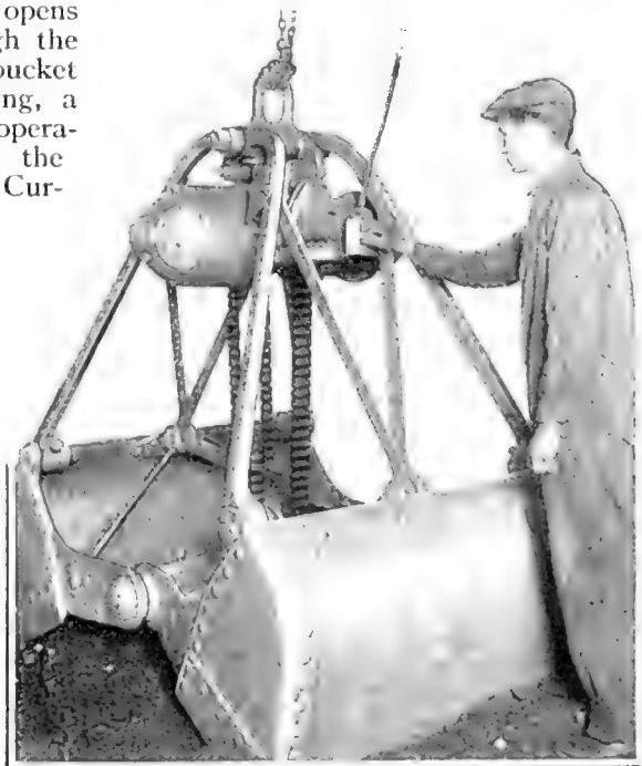
Note the motor on the clam-shell bucket. It opens and closes the two halves of the bucket with the aid of heavy chains. A multiple-hook prevents slipping
